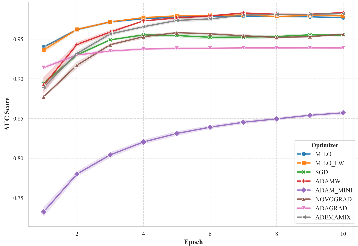
Validation AUC for RESNET34_CIFAR10 Experiment
